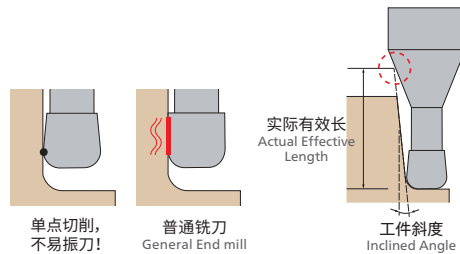
Suppress chattering by point milling (Dia.~2.5)
